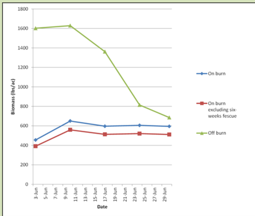
Above: Biomass totals from clipping (On burn) and VORs (Off burn) in Salt Flat.
